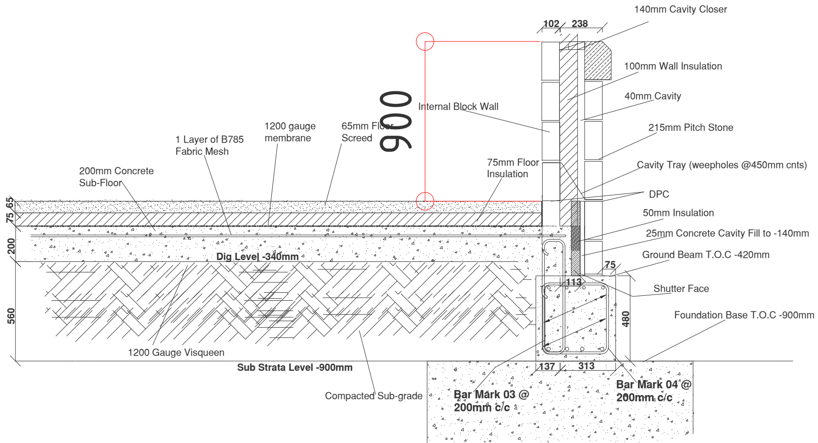
Section Through Floor Slab Perimeter (scale 1:20)
